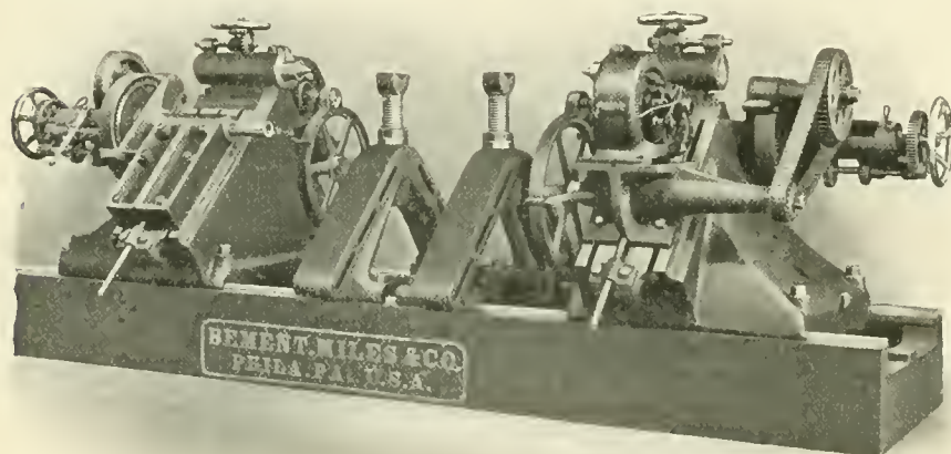
QUARTERING MACHINE—NILES-BEMENT-POND CO.
